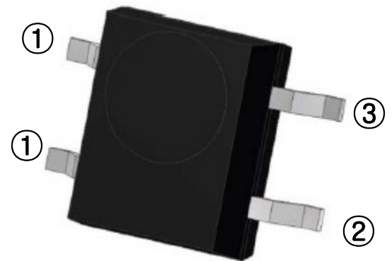
①=GND, ②=Output, ③=Vcc
